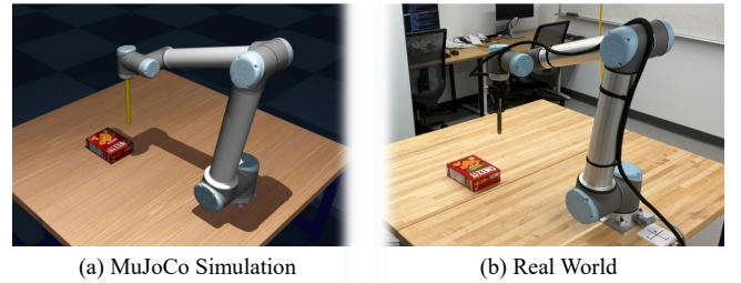
Fig. 4: Experiment Setup
