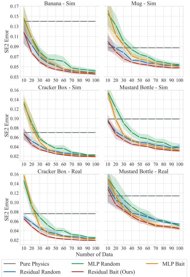
Fig. 5: Skill Learning results show SE(2) prediction error for 2 real objects, and 4 simulated objects from [24]: Banana, Mug, Cracker Box and Mustard Bottle. The active learning methods outperform random data collection, and models with residual physics performs better in low-data regime.
